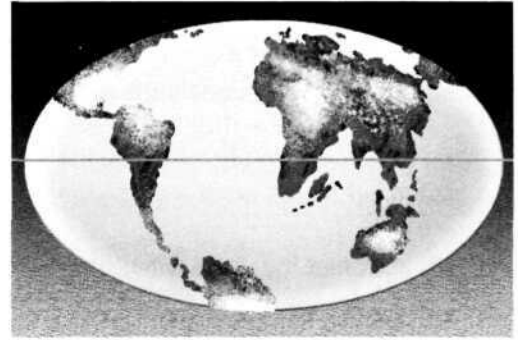
Our planet in 50 million years' time
