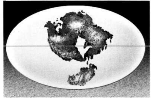
... and in 250 million years' time
